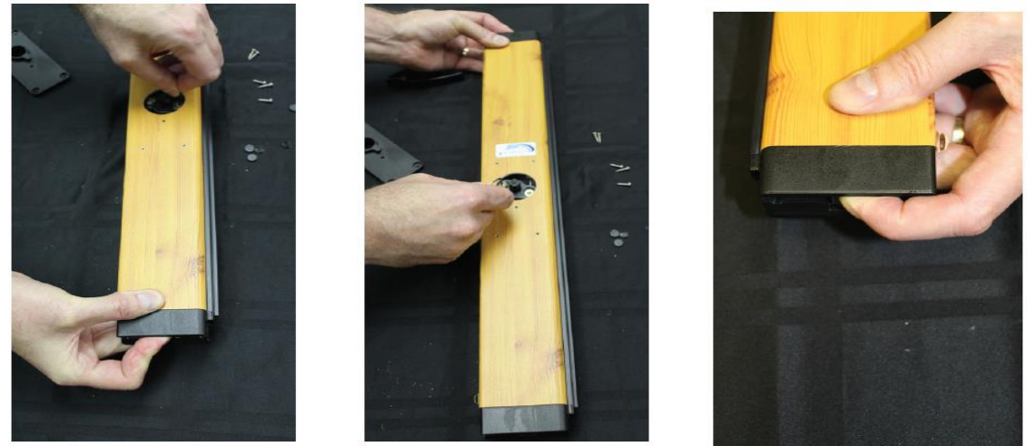
Step 4: Adjust the brakes on each end with Allen key so the caliper rests 1/8" inside each end-cap. Do this by pushing in on the calipers as tightening, install handle
