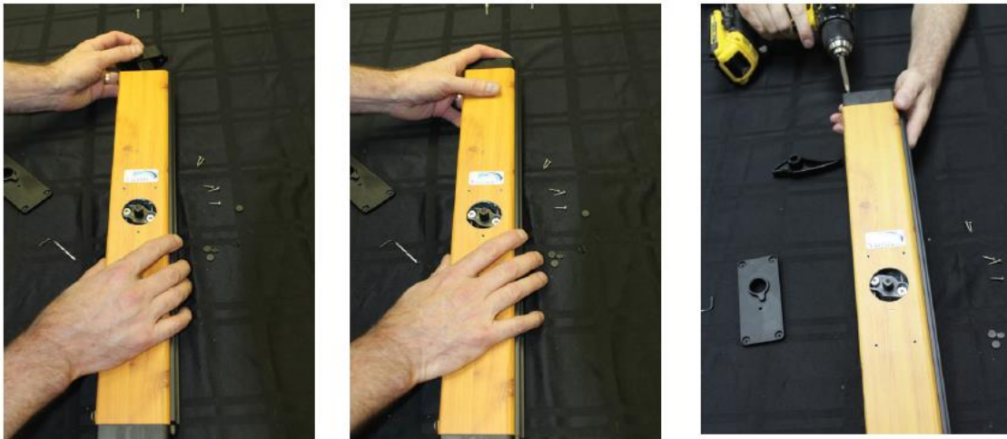
Step 3: Insert the upper endcap, fasten in place and proceed to set the brake calipers
